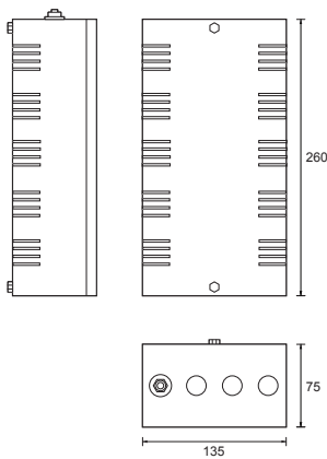
PS200T - 200W | PS300T - 300W
