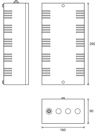
PS400T - 400W | PS500T - 500W
